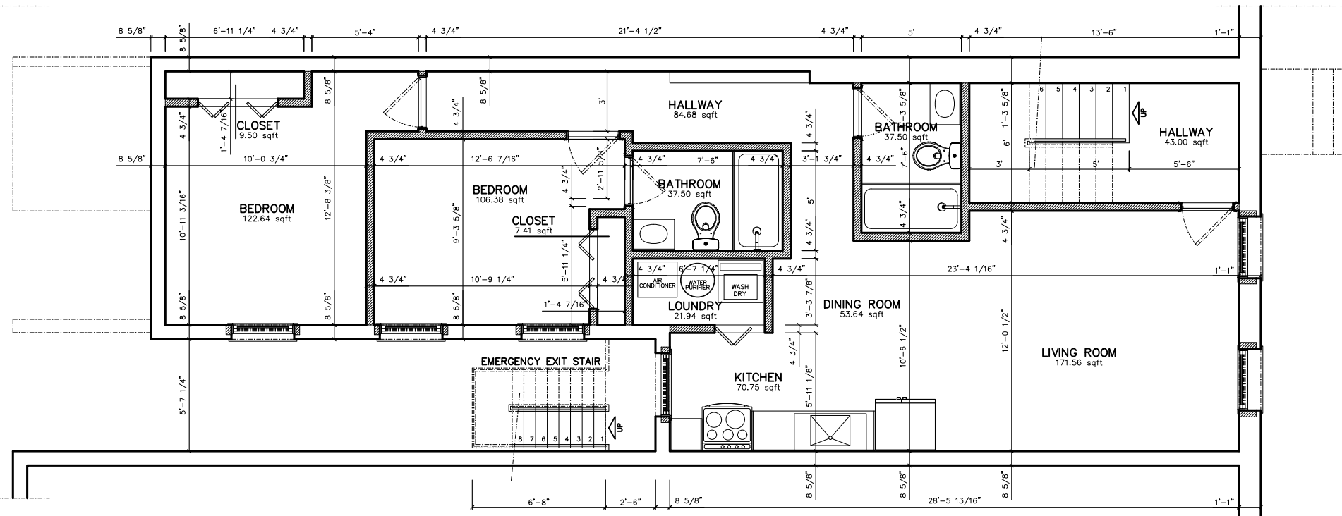
FLOOR PLAN BASEMENT
