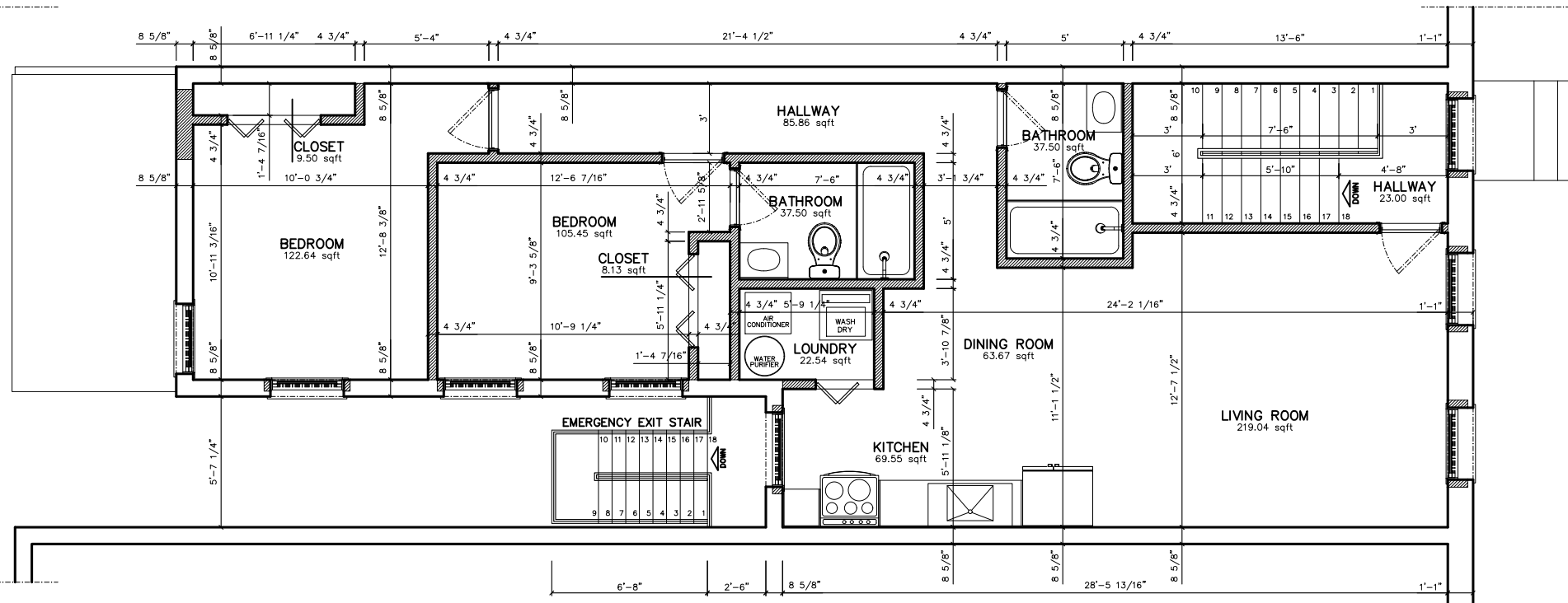
FLOOR PLAN 3rd FLOOR
