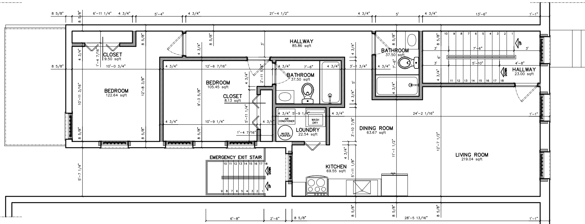
FLOOR PLAN 2nd FLOOR
